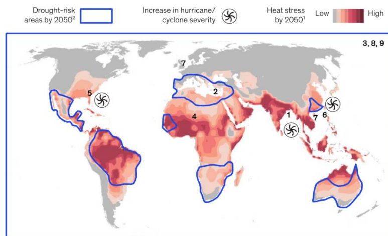
Figure 2 – Heat stress and drought-risk
